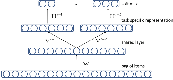
Fig. 1. The structure of Multi-task Representation Learning (MTRL) model. The lower two layers are shared across all the tasks, while top layers are task-specific. The input is represented as a bag of items. Then a non-linear projection \mathbf{W} is used to generate a shared representation. Finally, for each task, additional non-linear projection \mathbf{V} generates task-specific representations.
